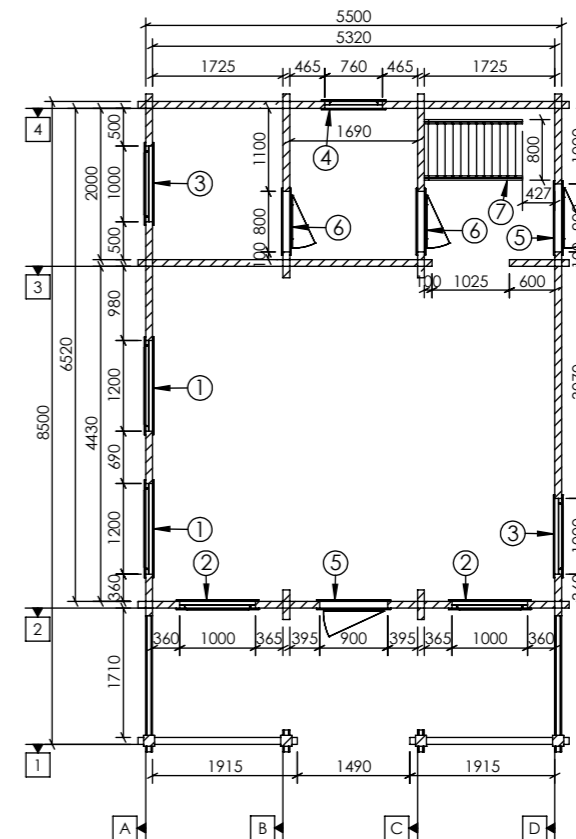
Plan
