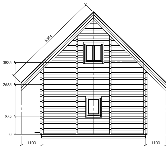
Facade D-A
