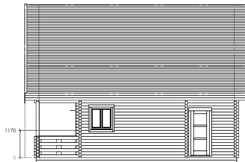
Facade 1-4
