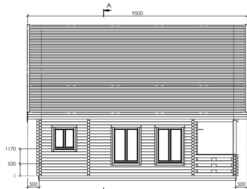
Facade 4-1
